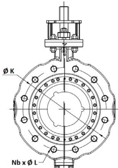
DN250
